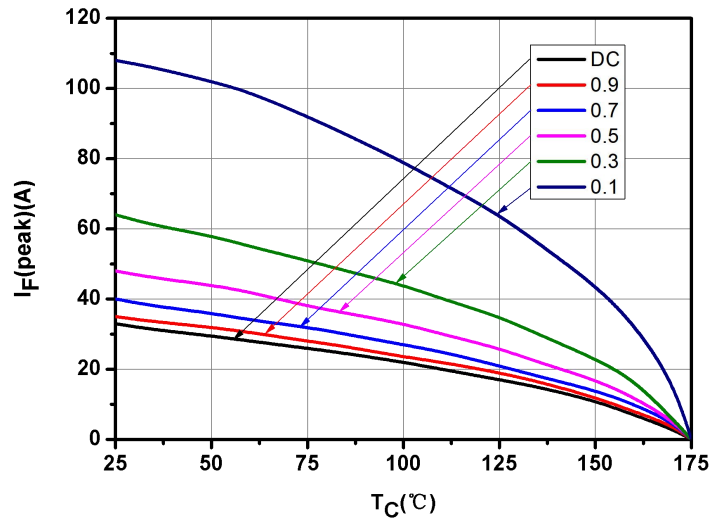
Fig.8-Current Derating
